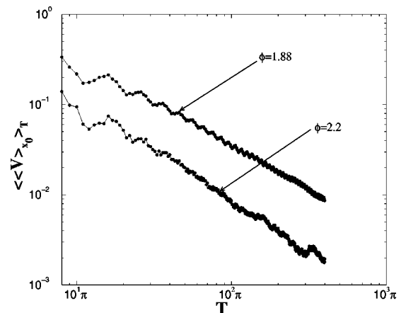
FIG. 3. An example of the power law decay of the mean velocity \langle \bar{V} \rangle_{X_0} inside the stochastic layer ( E_0 \approx 1 ) with increasing the time interval T at \phi \neq \phi_s ; \epsilon = 0.15 ; \omega = 1 .
